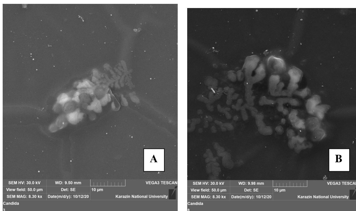
Figure 5. Scanning electronic microscopy of the daily biofilms of Candida albicans isolates under LED radiation of violet (A) and red (B) spectra with simultaneous action of Cu nanoparticles impregnated in non-woven polymeric material
