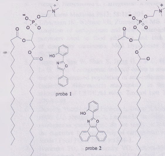
Figure 3. Expected location and orientation of fluorescent probes 1 and 2. Two molecules of phosphatidylcholine from the outer monolayer are shown to denote the location of the probes
