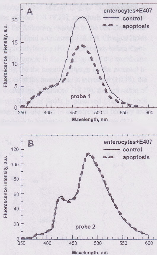
Figure 1. Fluorescence spectrum of probes 1 (panel A) and 2 (panel B) were recorded for: (I) the probes bound to enterocyte membranes from the control group of rats (solid line); (II) the probes bound to enterocyte membranes of animals with carrageenan-induced gastroenterocolitis in condition of activation of apoptotic processes (dashed line)
