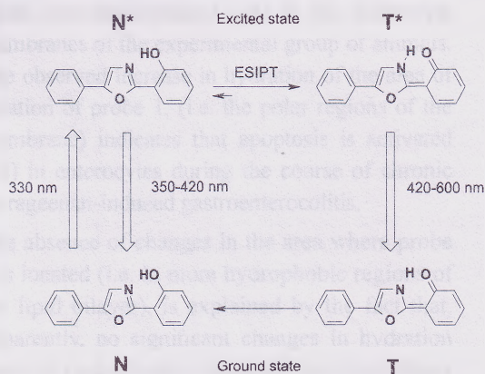
Figure 2. Scheme of excited state intramolecular proton transfer (ESIPT) in 2-(2'-hydroxyphenyl)-5-phenyl-1,3-oxazole (probe 1). The upwards arrow shows the electronic excitation and the downwards arrow represents the emission of light (fluorescence). Corresponding maximum of absorption and the ranges of emission are measured in nanometres
